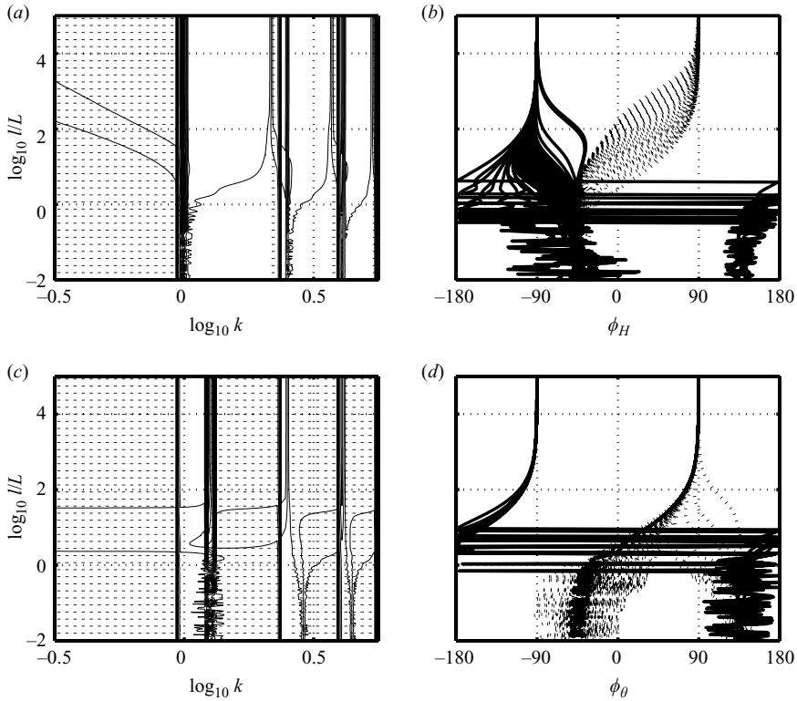
FIGURE 10. Contour plots of the optimal-efficiency phases for (a, b) the driving amplitude H_0 and (c, d) the pitching angle \Theta_0 . The phase with zero phase centred on the body's trailing edge is shown in (a) and (c). The variation of phase along vertical lines in (a) and (c) is shown in (b) and (d). The dotted lines give the phases for the dotted regions in (a) and (c); the solid lines give the phases in the remaining regions.
